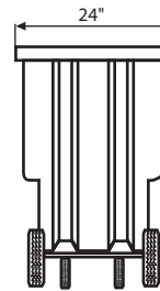
½ Yard Dump Cart with 10" Wheels
