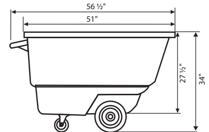
½ Yard Dump Cart with 10" Wheels
