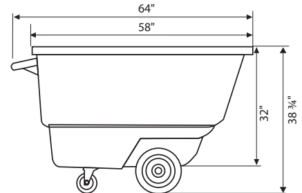
Dump Cart with Full Frame & 12" Wheels
