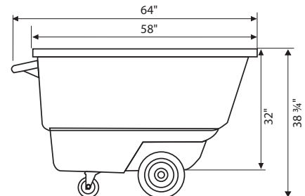
Dump Cart with 12" Wheels
